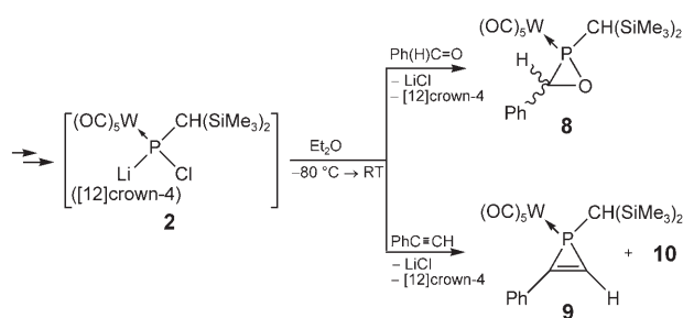
Scheme 4. Reaction of complex 2 with \text{Ph(H)CO} or \text{PhC}\equiv\text{CH} .
