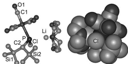
Figure 2. Gas-phase DFT structure of complex 2 ; ball-and-stick model (left) and space-filling model (right). Selected bond lengths [Å] and angles [°]: W–P 2.652, P–Cl 2.217, P–Li 2.652, P–C2 1.905, Cl–Li 3.465, W–Cl 2.011, C1–O1 1.154; Cl–P–W 110.43, Cl–P–C2 101.45, W–P–C2 112.03, \Sigma \angle P 323.91°. Charges from a natural population analysis (Mulliken charges in brackets) of Hartree–Fock orbitals: P +0.248 (+0.162), W –0.963 (+0.733), Cl –0.462 (–0.460), C2 –1.515 (–1.227), C1 +0.678 (–0.039), O1 –0.606 (–0.314), Li +0.853 (+0.816).
