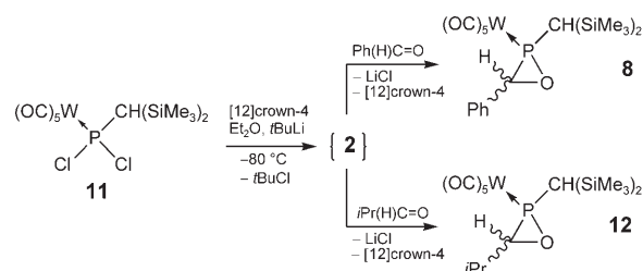
Scheme 5. Simpler access to complex 2 .
