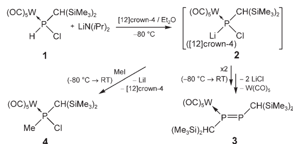
Scheme 2. Generation and reactions of complex 2 .
