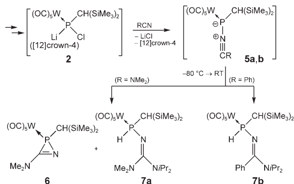
Scheme 3. Reaction of complex 2 with nitriles.
