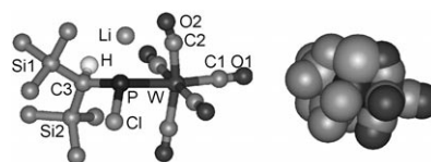
Figure 1. DFT gas-phase structure of 2' (without [12]crown-4; B3LYP/6-311g(d,p), LanL2DZ at W); ball-and-stick model (left) and space-filling model (right). Selected bond lengths [Å] and angles [°]: W-P 2.631, P-Cl 2.160, P-Li 2.416, Cl-Li 3.774, P-C3 1.890, W-C1 2.024, W-C2 1.987, C1-O1 1.149, C2-O2 1.181; W-C2-O2 164.71, Cl-P-W 112.31, Cl-P-C3 103.65, W-P-C3 122.21, \Sigma \angle \text{P} 338.17°. Charges from a natural population analysis (Mulliken charges in brackets) of Hartree-Fock orbitals: P +0.201 (+0.203), W -0.933 (+0.773), Cl -0.401 (-0.358), C3 -1.502 (-1.198), C1 +0.688 (-0.028), O1 -0.578 (-0.288), C2 +0.680 (+0.064), O2 -0.743 (-0.429), Li +0.906 (+0.599).
